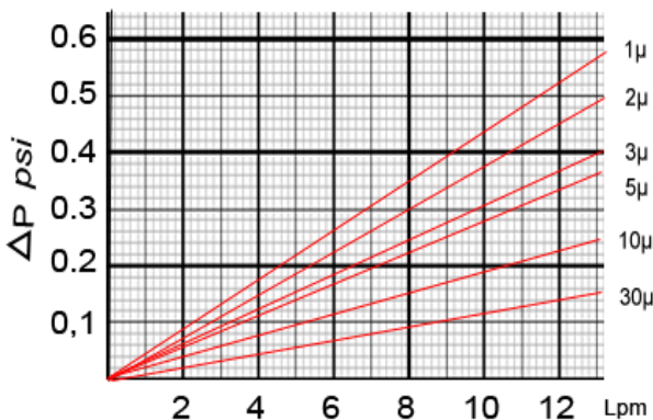
For single 10" cartridge length indicative of clean differential pressure
